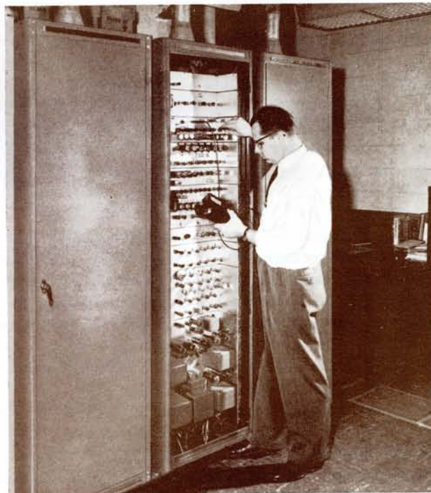
Above, the Phonevision sound coder. Scrambling the picture alone is not sufficient. Sound must be scrambled also to prevent unauthorized reception by a non-subscriber.
